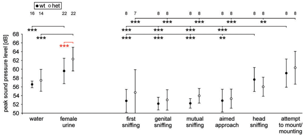
Figure 8: Peak sound pressure level (dB SPL) of USVs. The average peak SPLs of USVs (mean \pm SD) are shown for both groups (wt, het) and the indicated experimental situations. Female urine led to significantly louder USVs than water. USVs recorded during head sniffing and attempt to mount/mounting interactions were often significantly louder than USVs from the other female interactions. Het group animals had louder USVs than wt group animals in response to female urine. For further explanations see Fig. 1.
