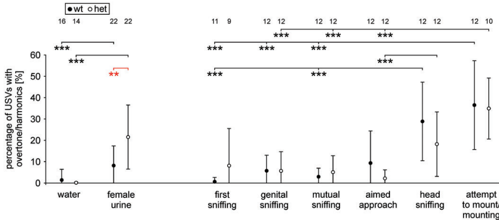
Figure 9: Percentage of USVs with overtones or harmonics. The average percentages of USVs with overtones or harmonics (mean \pm SD) are shown for both groups (wt, het) and the indicated experimental situations. Female urine led to significantly more USVs with overtone/harmonics than water. USVs recorded during head sniffing and attempt to mount/mounting interactions had often significantly more overtone/harmonics than USVs from the other female interactions. Het group animals had higher percentages of USVs with overtones/harmonics than wts in response to female urine. Statistical comparisons in the experiments with water and female urine and in the interaction experiment had Bonferroni adjustment. For further explanations see Fig. 1.
